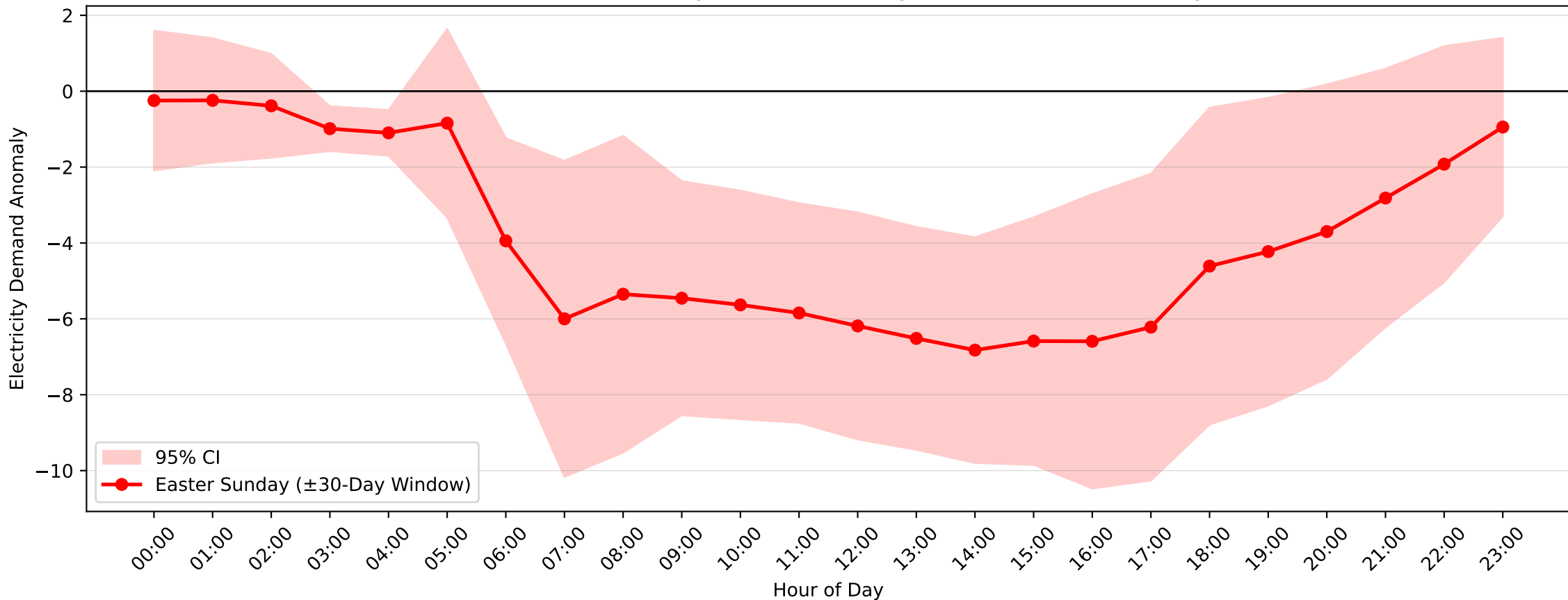
Chatswood Demand Anomaly: Easter Sunday (2004–2017, \pm 30 -Day Window)
